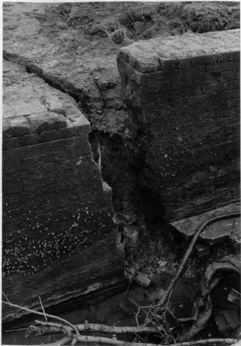
Broken Clayhole culvert revealed while pumping from Clayhole. November, 1961.
